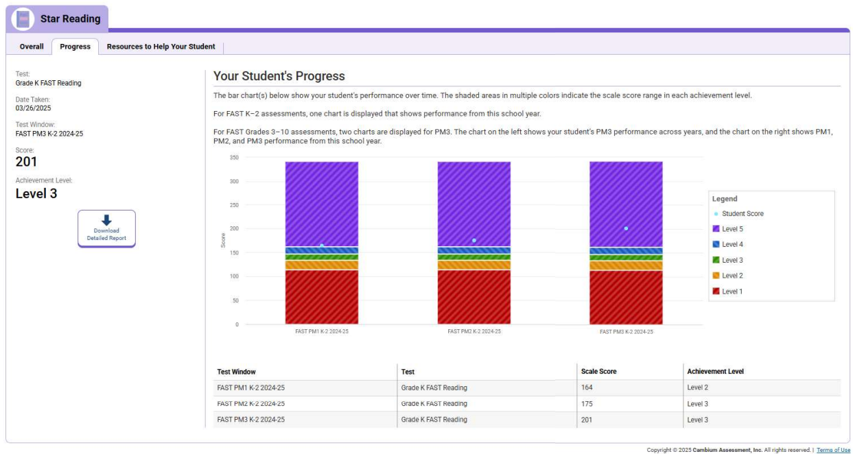
Figure 4. Progress Tab
